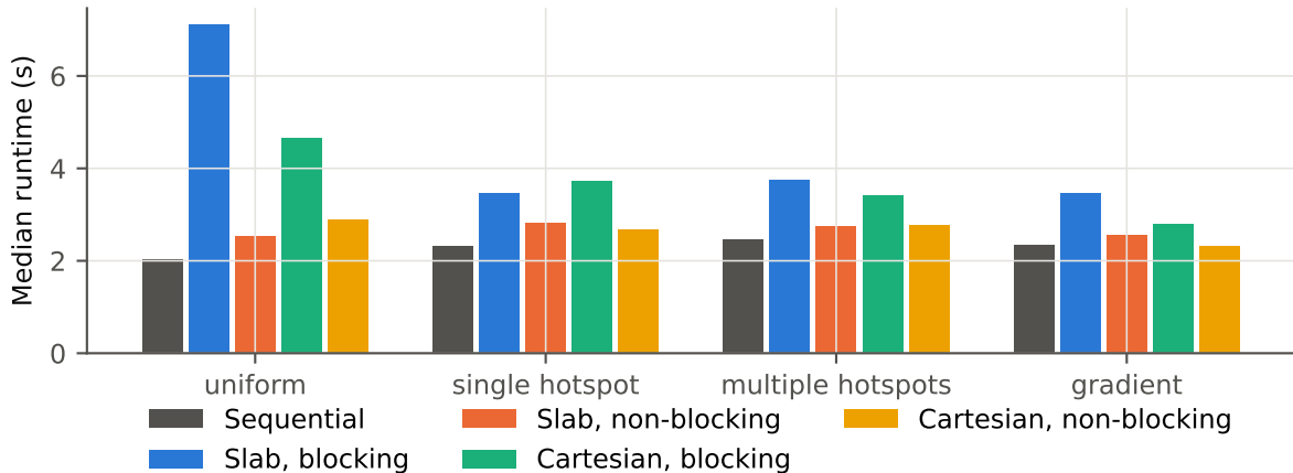
Runtime by scenario, 1000 x 1000, MPI variants on 2 processes
